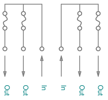
Circuit diagram: 2 inputs and 4 "fused" outputs
